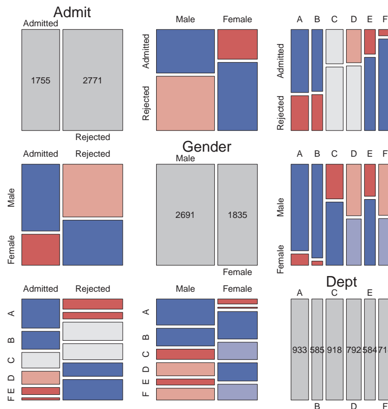
{fig:berk-pairs1} Figure 5.24: Mosaic matrix of the UCBA admissions data showing bivariate marginal relations.
