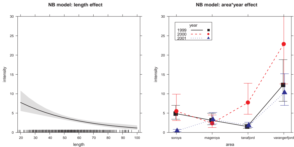
{fig:cod3-eff1} Figure 11.22: Effect plots for total intensity of parasites from the negative-binomial model.
