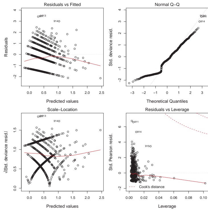
{fig:phdpubs5-plot} Figure 11.33: Default diagnostic plots for the negative-binomial model fit to the PhdPubs data.
