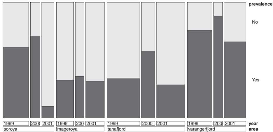
Figure 11.16: Doubledecker plot for prevalence against area and year in the CodParasites data. The cases of infected fish are highlighted.
