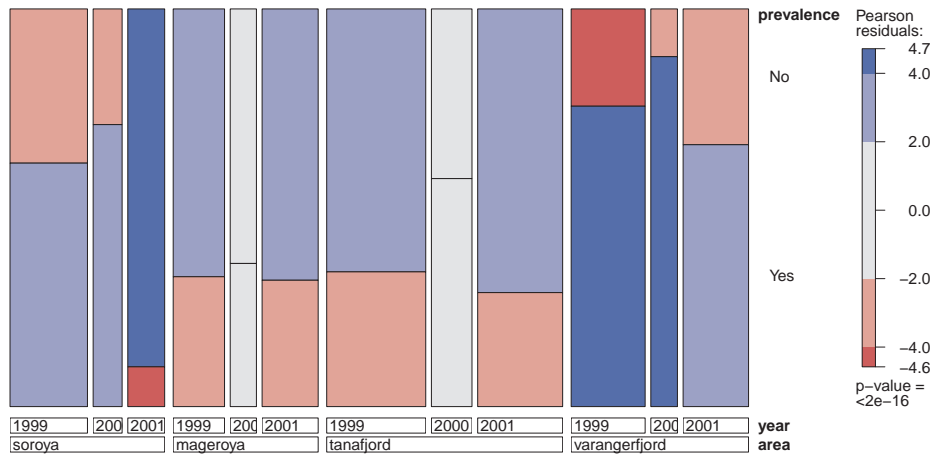
Figure 11.17: Mosaic plot for prevalence against area and year in the CodParasites data, in the doubledecker format. Shading reflects departure from a model in which prevalence is independent of area and year jointly.
