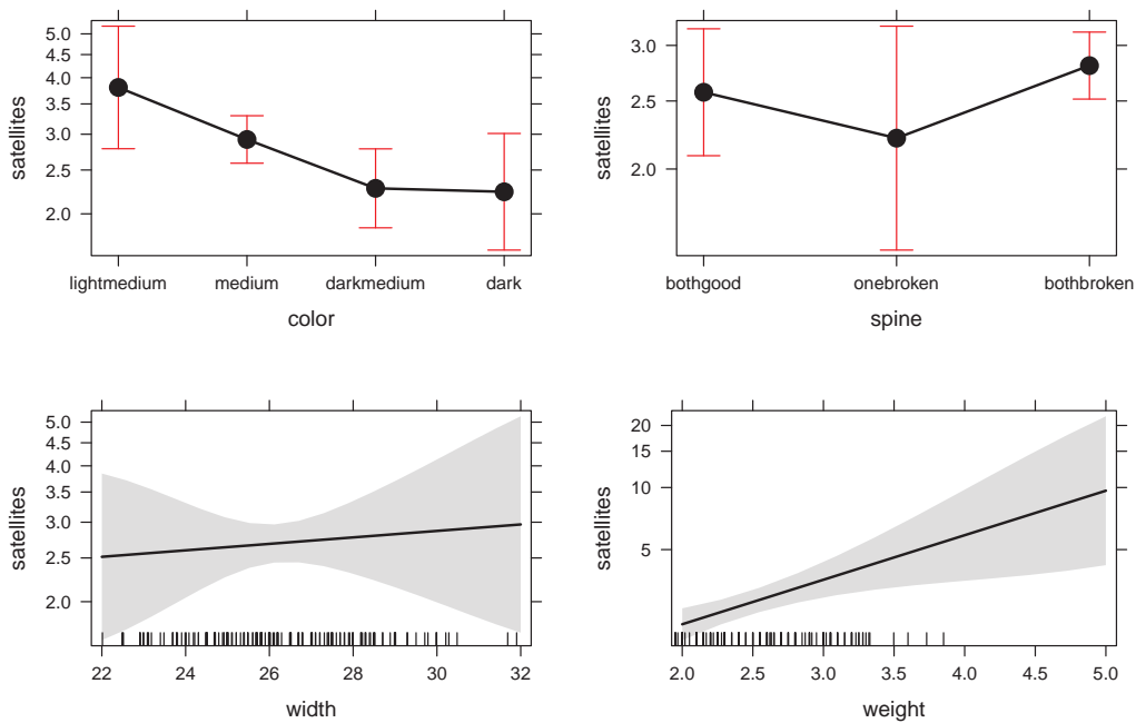
Figure 11.7: Effect plots for the predictors in the Poisson regression model for the CrabSatellites data. {fig:crabs1-eff1}
