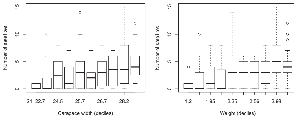
Figure 11.6: Boxplots of number of satellites vs. width and weight.
