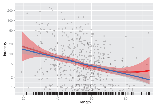
Figure 11.20: Jittered scatterplot of \log(\text{intensity}) for the positive counts against length of fish, with loess smooth and linear regression line.
